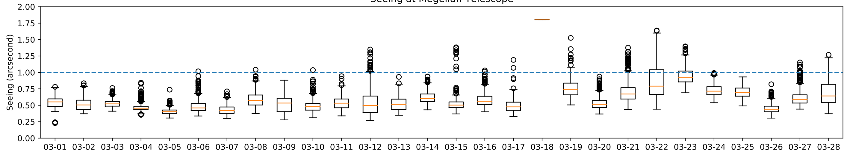
Seeing at Megellan Telescope
